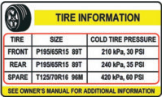
Figure 2: EXAMPLE—Tire Information Placard
